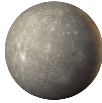
Mercury
