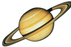
Saturn
