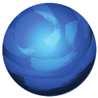
Neptune
