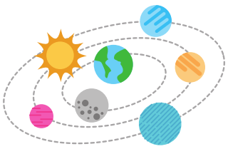
solar system
